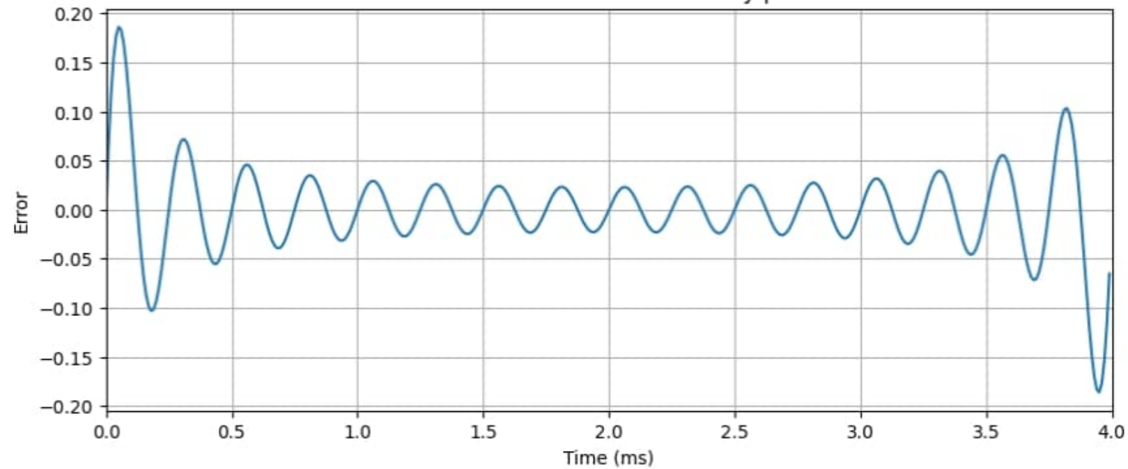
Reconstruction Error - Above Nyquist
