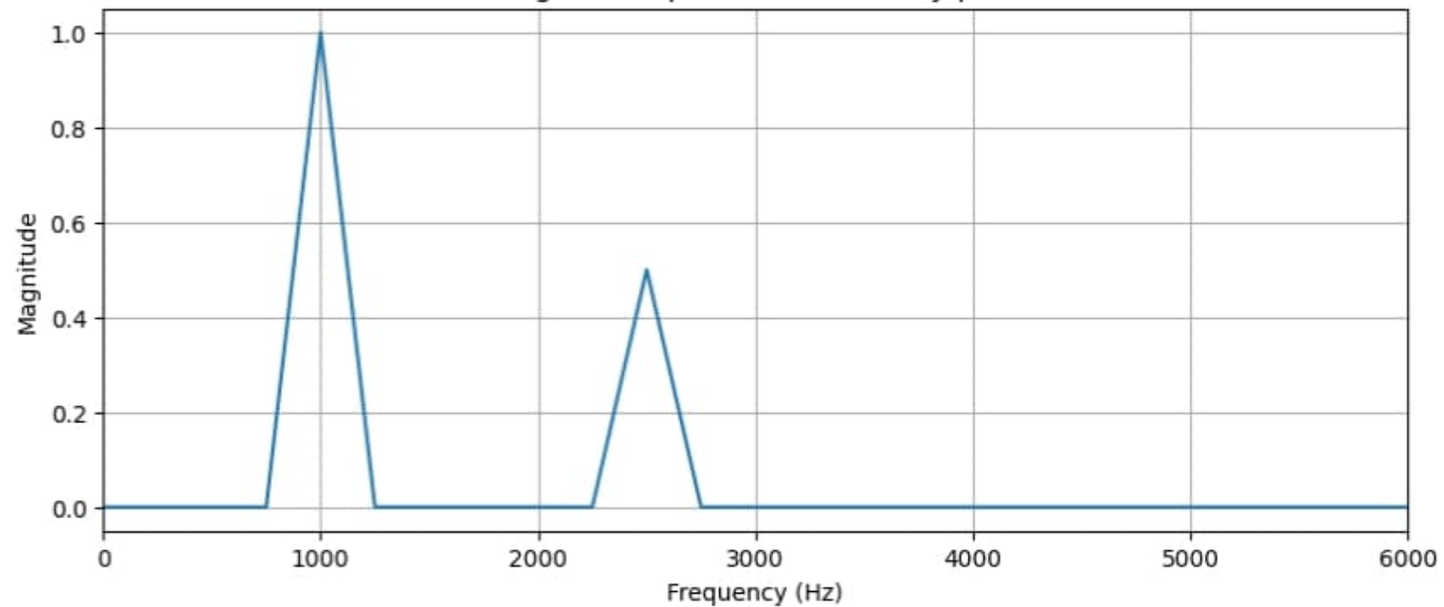
Magnitude Spectrum - Above Nyquist
