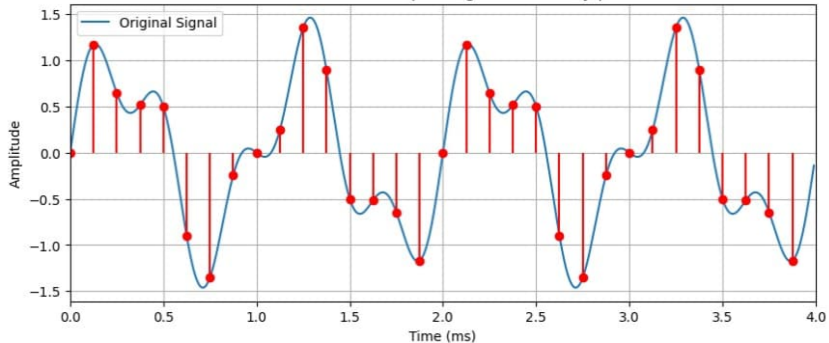
Reference and Sampled Signal - Above Nyquist
