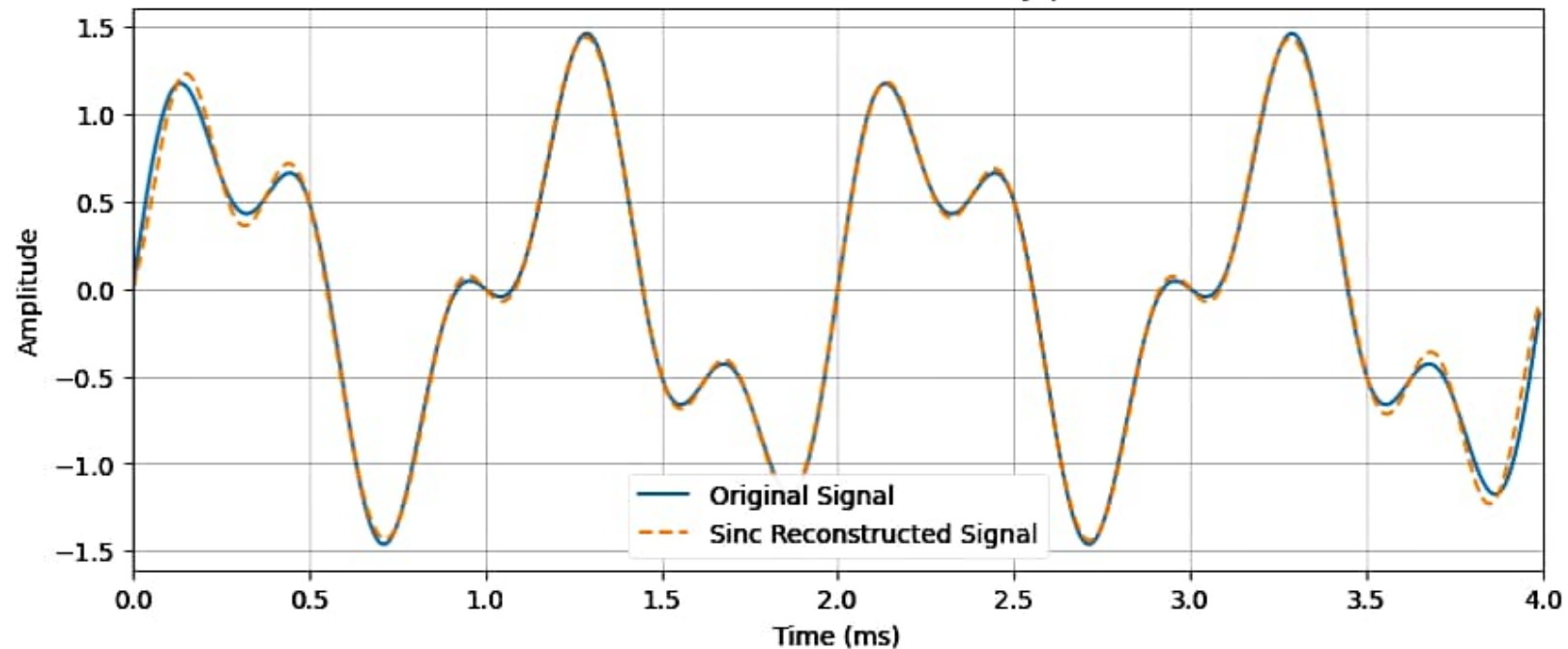
Sinc Reconstruction - Above Nyquist
